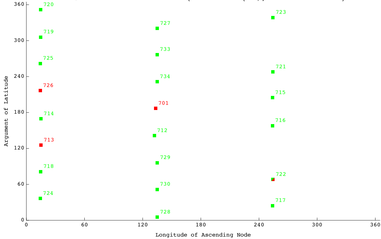
GLONASS Satellite Constellation (GPS Week 1570(546) ; GPS Seconds 345 600)
